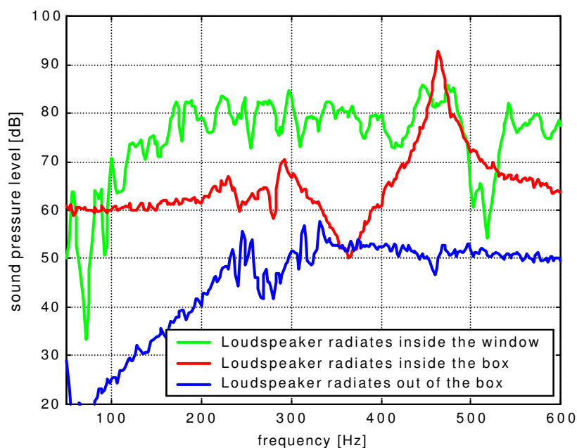
Fig. 4: Frequency responses of the loudspeaker radiating outside and inside a rigid box and radiating inside the double-glazed window
