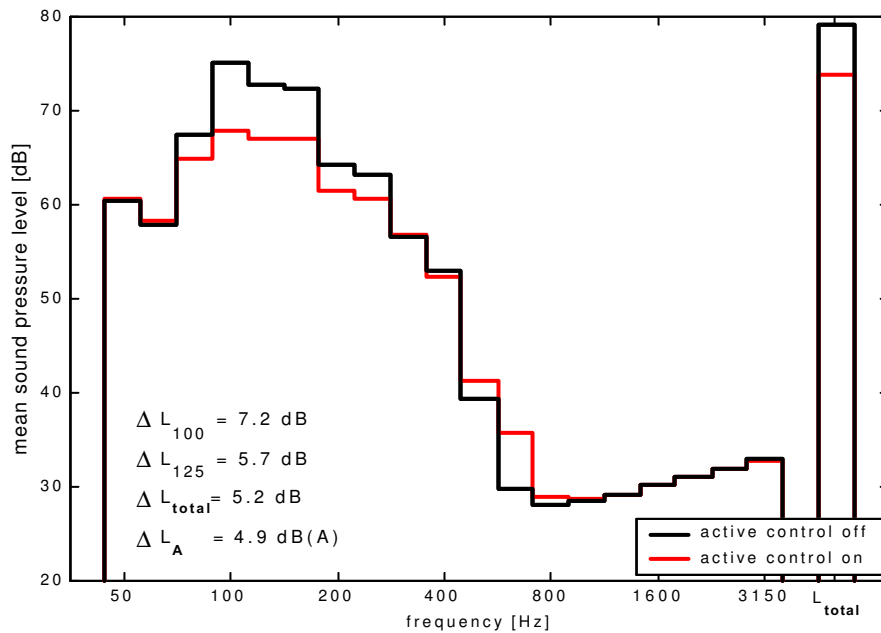
Fig. 6: Third-octave band mean sound pressure levels measured in the receiving room without and with active control for band-limited white noise excitation
