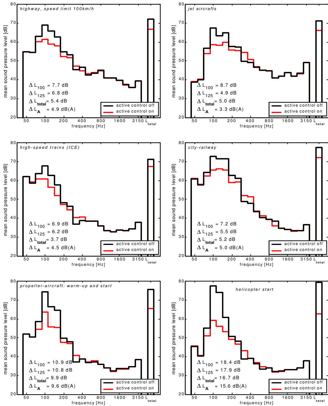
Fig. 7: Third-octave band mean sound pressure levels measured in the receiving room without and with active control for different traffic noise examples
