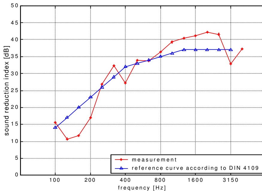
Fig. 2: Sound reduction index of the window without active control
