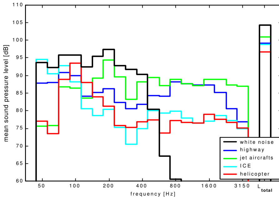
Fig. 5: Sound pressure levels of the noise excitation measured directly in front of the outer side of the active window
